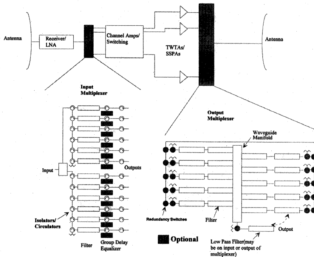
Fig. 1. Simplified block diagram of a communication satellite payload, illustrating the function of the input and output multiplexers (filter banks).
