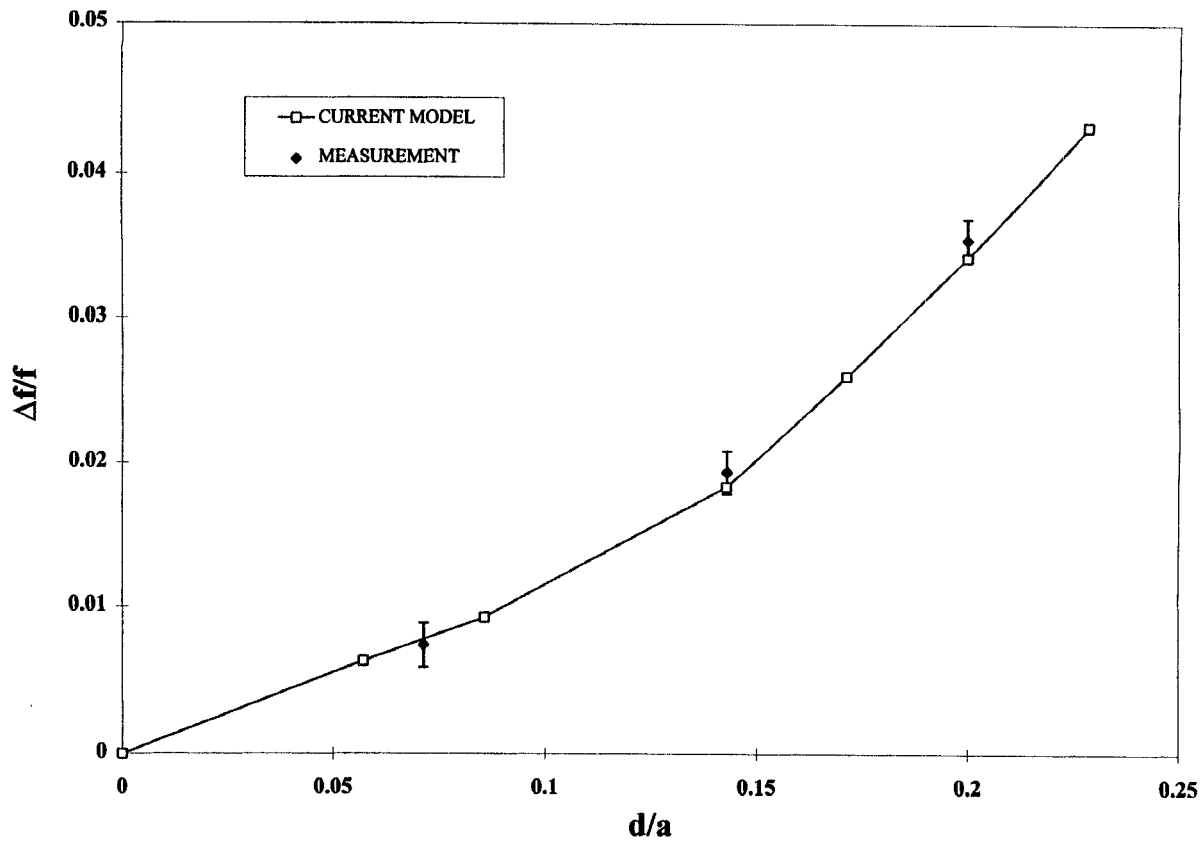
Fig. 9. Comparison of calculated and measured results for the modeling approach presented herein for dual mode planar resonators.
