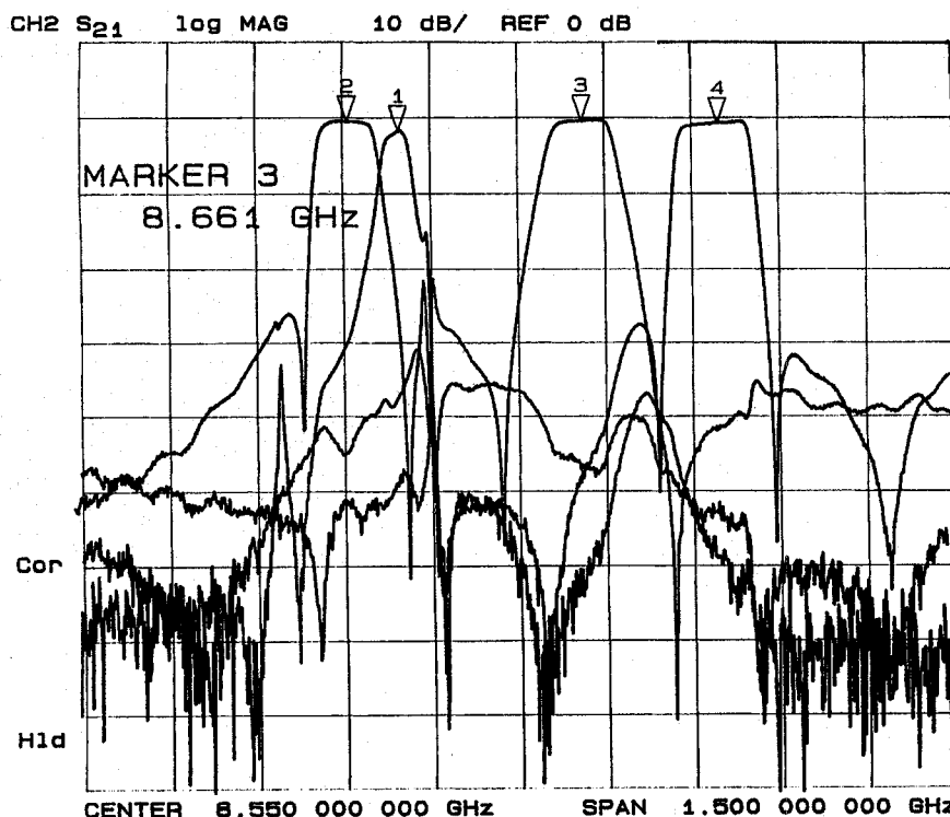
Fig. 15. Measured performance of the HTSSE-II multiplexer shown in Fig. 14. The performance matched with the theoretical analysis reasonably well. The narrow channel simulates a beacon as is commonly used in communication satellite multiplexers.
