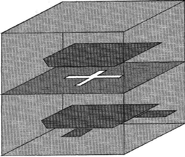
Fig. 7. Illustration of a four-pole dual mode planar filter in a stacked configuration. This filter is made from two dual mode stripline resonators that are vertically stacked and coupled together through an iris in their common ground plane.
