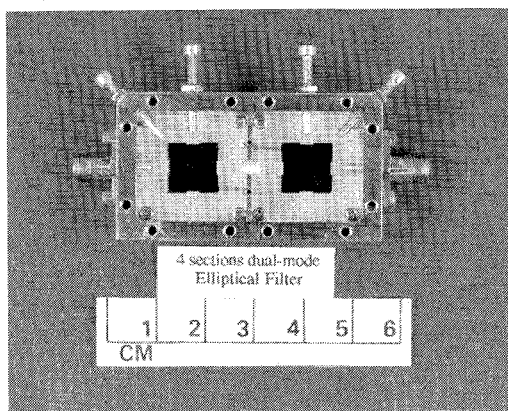
Fig. 10. Photograph of a dual mode suspended substrate HTS filter. Four of these filters were integrated to a multiplexer for the HTSSE-II.
