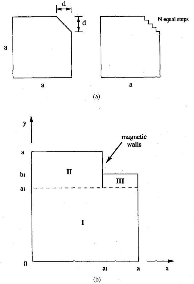
Fig. 8. Modeling of dual mode planar filters is illustrated. (a) Cut away corner section is modeled as a series of N steps. (b) N = 1 step.
