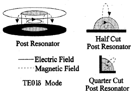
Fig. 2. Illustration of post dielectric resonator and their corresponding electromagnetic field configurations.
