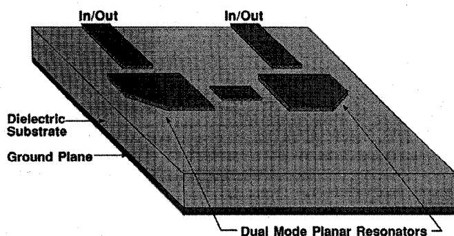
Fig. 6. Illustration of a four-pole, dual mode Chebyshev filter in a microstrip configuration.
