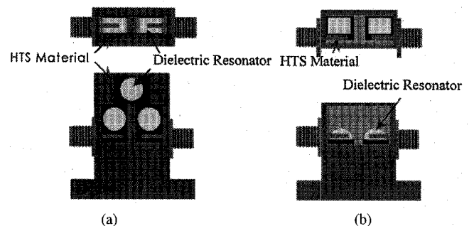
Fig. 3. Sketches of single mode, dielectric/HTS resonator filters including: (a) post resonator and (b) half-cut resonator.
