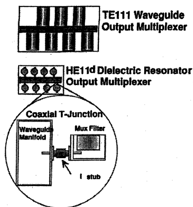
Fig. 12. Illustration of a conventional dielectric resonator multiplexer in comparison to a multiplexer based on cavity filters. The waveguide/coaxial/filter connection concept illustrated here is employed on the HTS multiplexer built for HTSSE-II.
