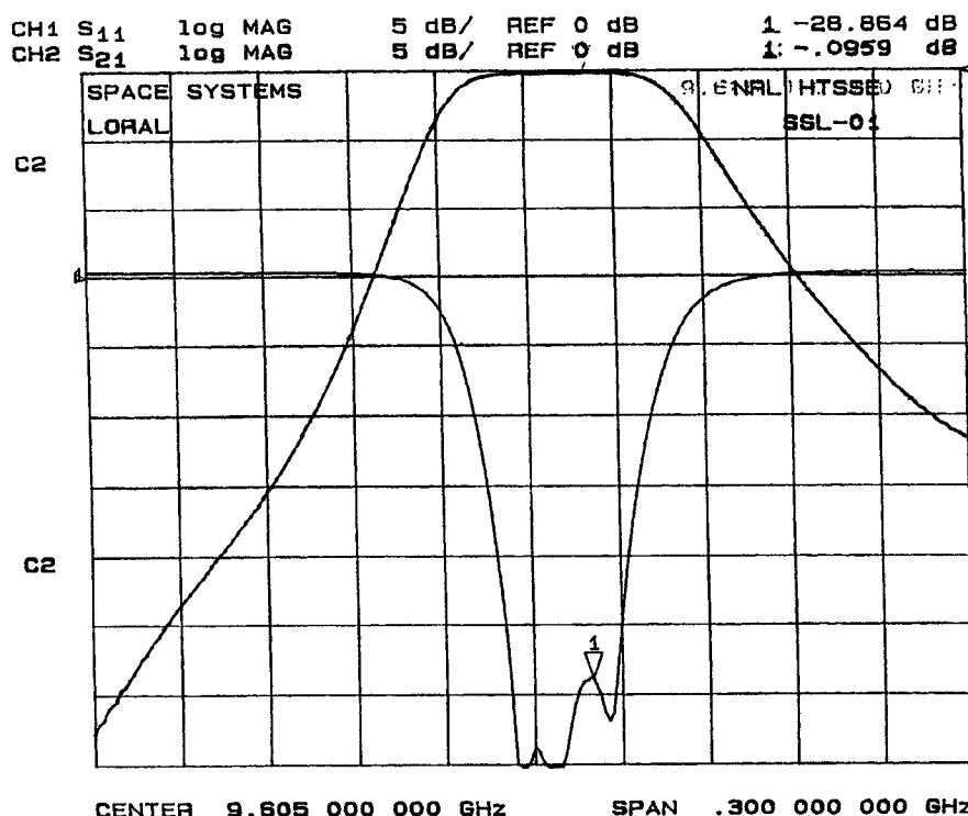
Fig. 4. Measured insertion loss and return loss performance of a three-pole, single mode dielectric/HTS resonator filter developed for HTSSE-I.
