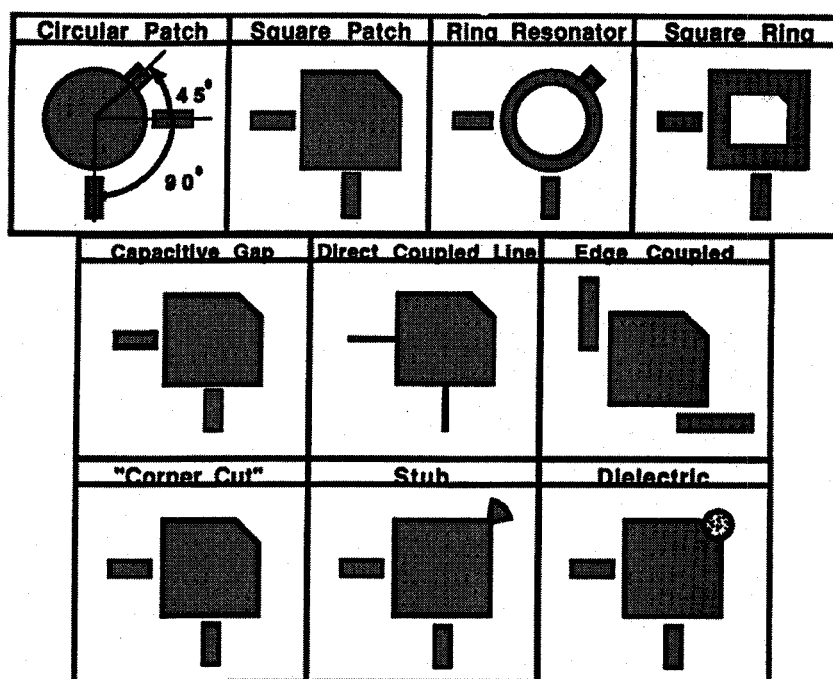
Fig. 5. Building blocks of dual mode planar HTS filters. The top row illustrates the resonator structures, the middle row illustrates coupling to the resonators, and the bottom row illustrates possible perturbations to the resonators to accomplish coupling between the dual orthogonal modes.
