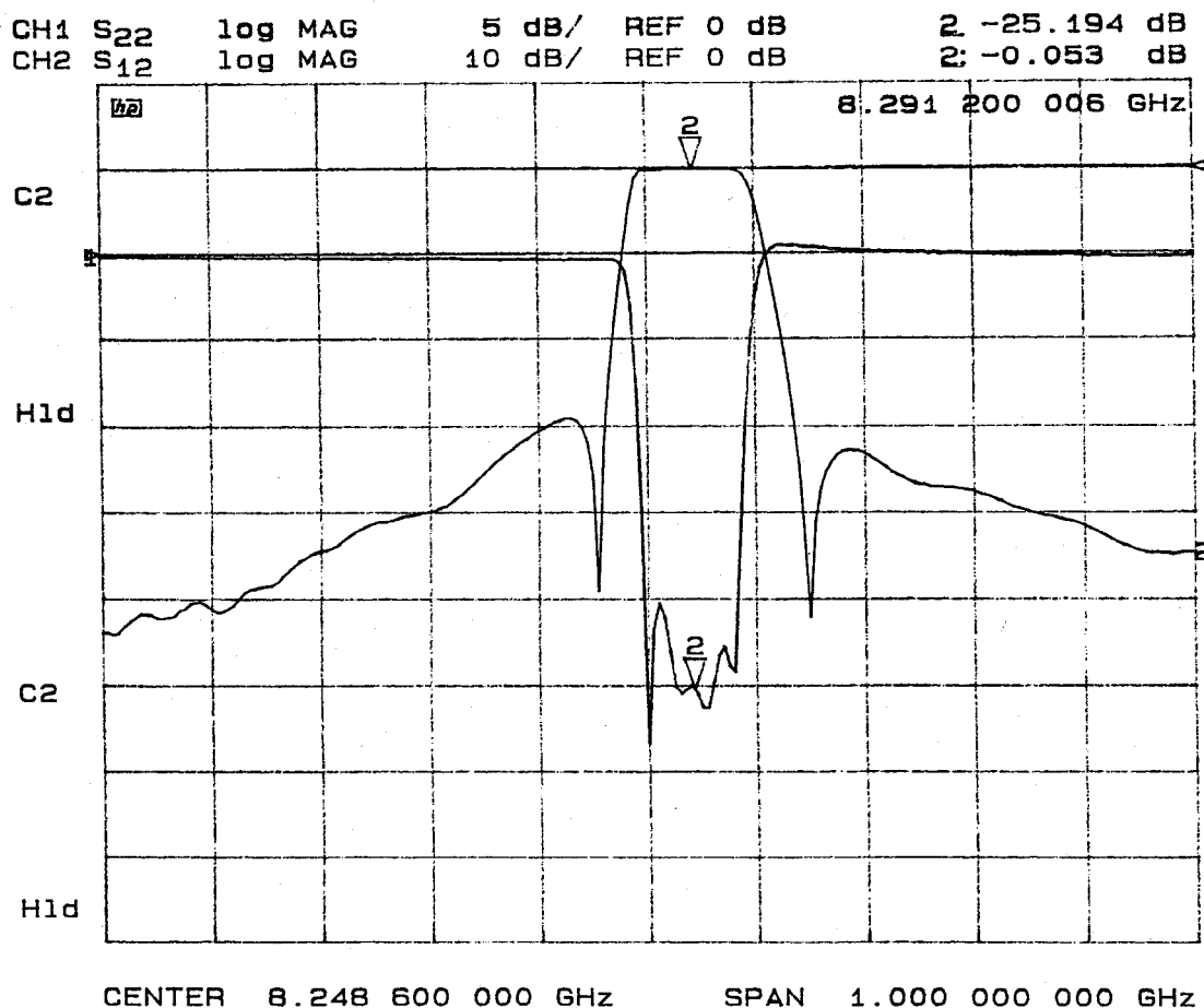
Fig. 11. Measured rejection and return loss performance of the HTSSE-II filter illustrated in Fig. 10.
