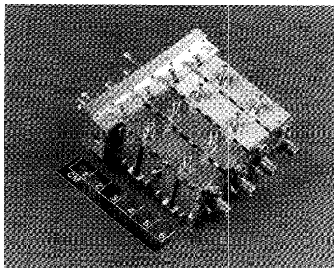
Fig. 14. Photograph of the waveguide/probe coupled HTSSE-II multiplexer based on dual mode, suspended substrate HTS filters.
